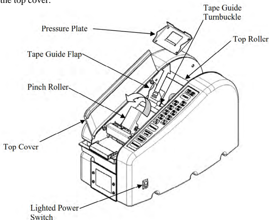
Figure 2 – Loading Tape
